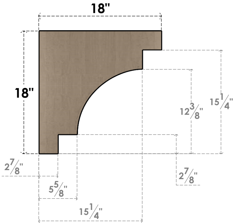
SIDE PROFILE
